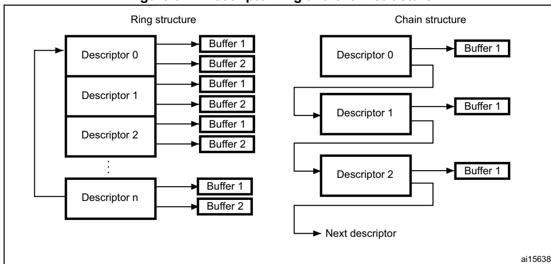
Figure 512. Descriptor ring and chain structure
