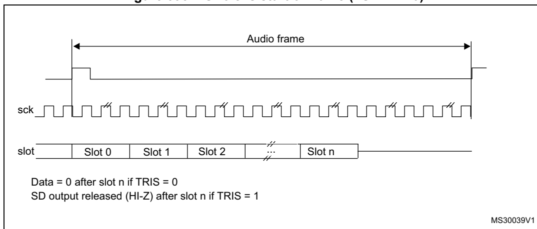
Figure 395. FS role is start of frame (FSDEF = 0)
