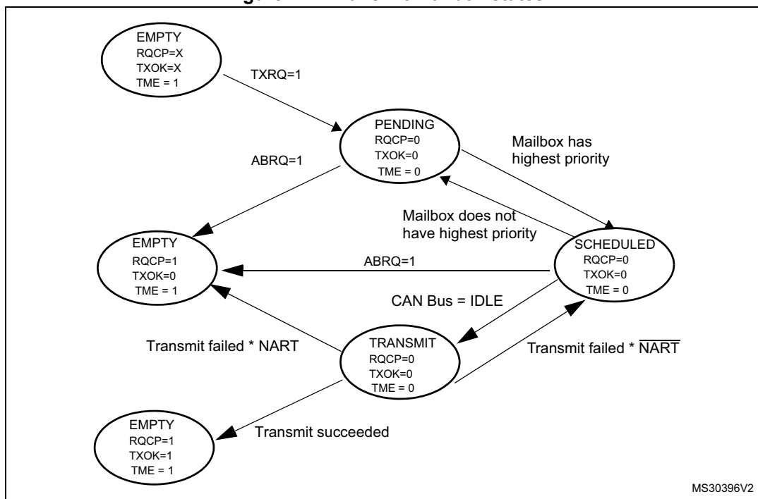
Figure 444. Transmit mailbox states
