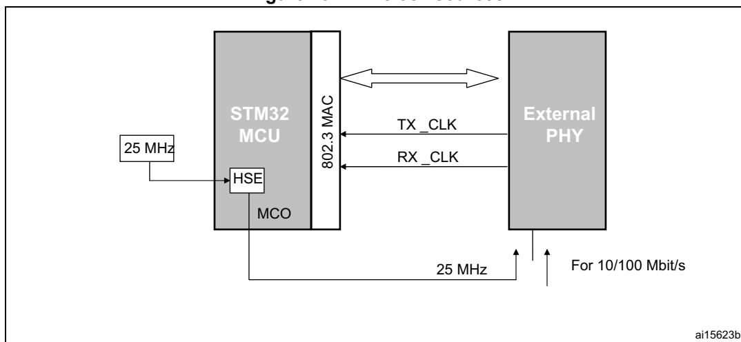
Figure 491. MII clock sources
