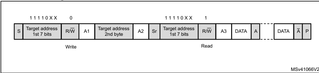
Figure 314. 10-bit address read access with HEAD10R = 0
