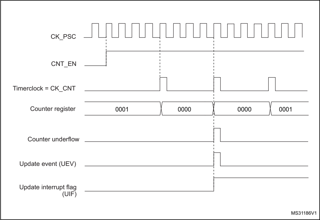
Figure 214. Counter timing diagram, internal clock divided by 4
