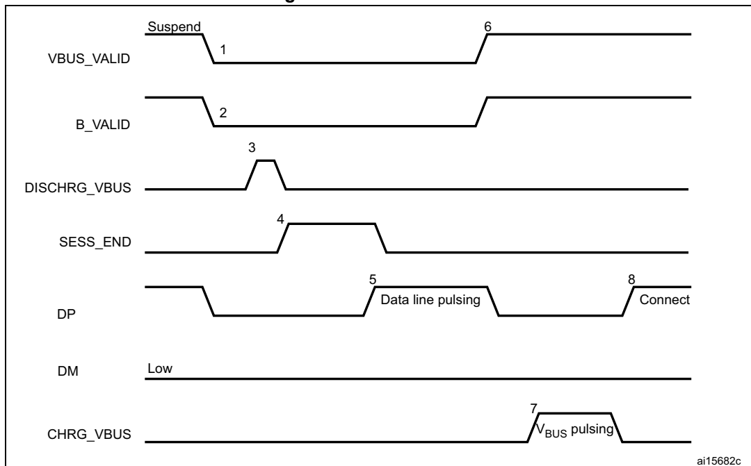
Figure 483. B-device SRP
