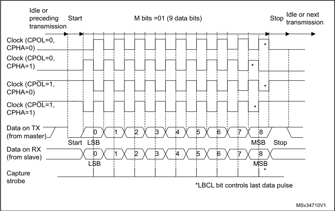
Figure 342. USART data clock timing diagram (M bits = 01)
