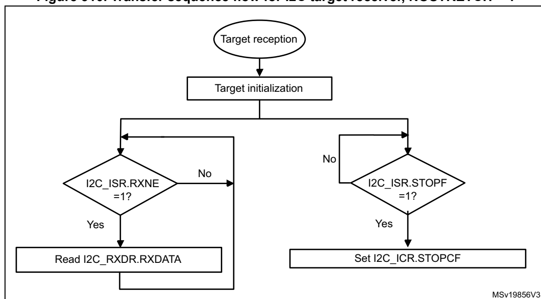
Figure 310. Transfer sequence flow for I2C target receiver, NOSTRETCH = 1
