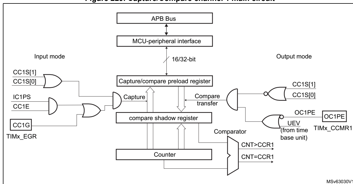
Figure 229. Capture/Compare channel 1 main circuit
