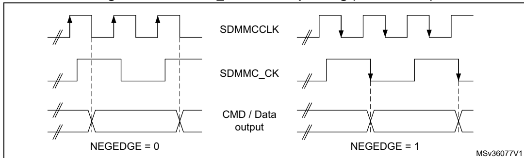
Figure 432. SDMMC_CK clock dephasing (BYPASS = 0)
