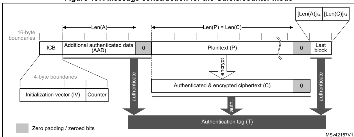
Figure 137. Message construction for the Galois/counter mode
