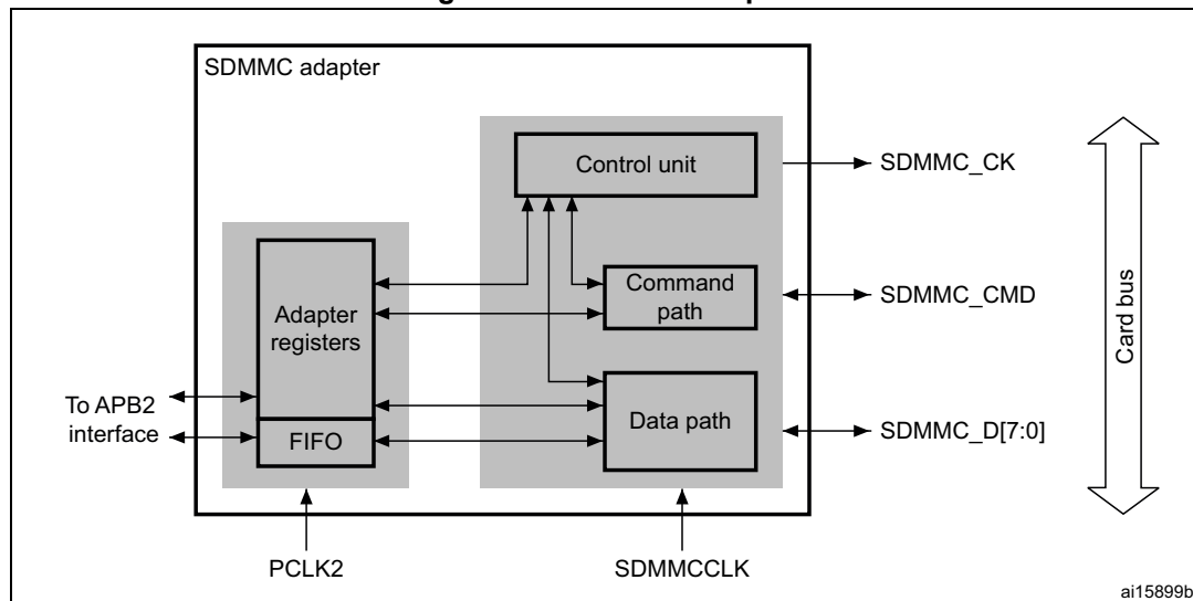
Figure 430. SDMMC adapter
