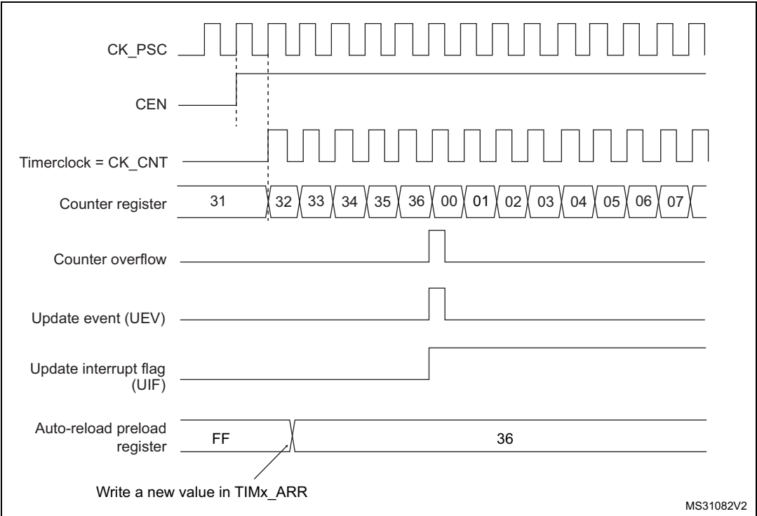
Figure 261. Counter timing diagram, update event when ARPE=0 (TIMx_ARR not preloaded)
