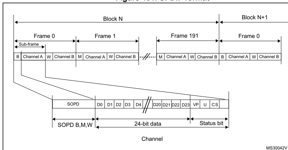
Figure 401. SPDIF format
