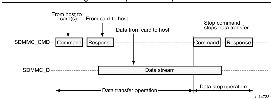
Figure 427. Sequential read operation
