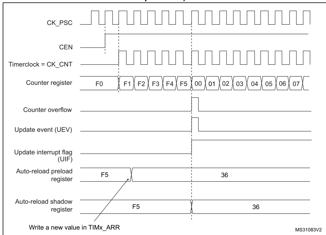
Figure 211. Counter timing diagram, Update event when ARPE=1 (TIMx_ARR preloaded)
