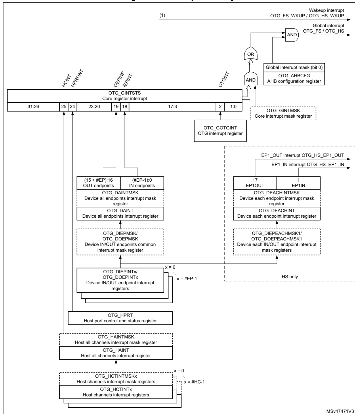
Figure 463. Interrupt hierarchy
