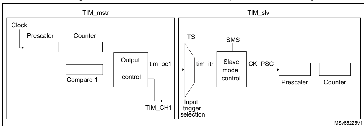
Figure 247. Master/slave connection example with 1 channel only timers
