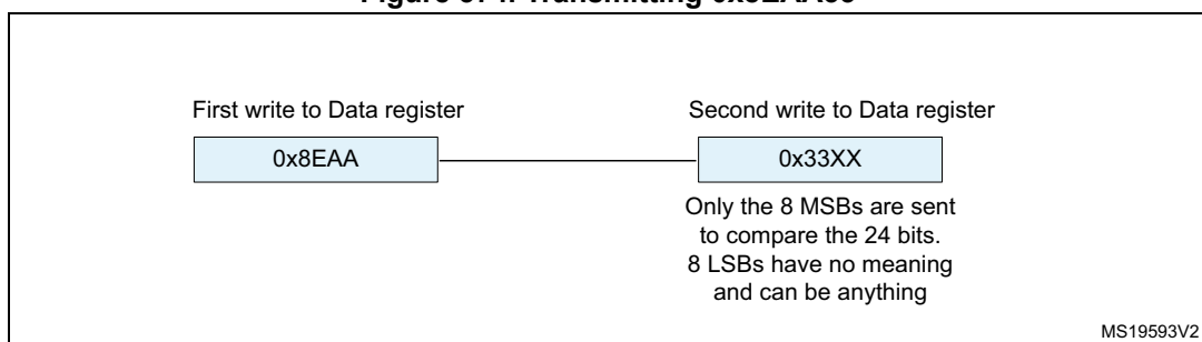
Figure 374. Transmitting 0x8EAA33
