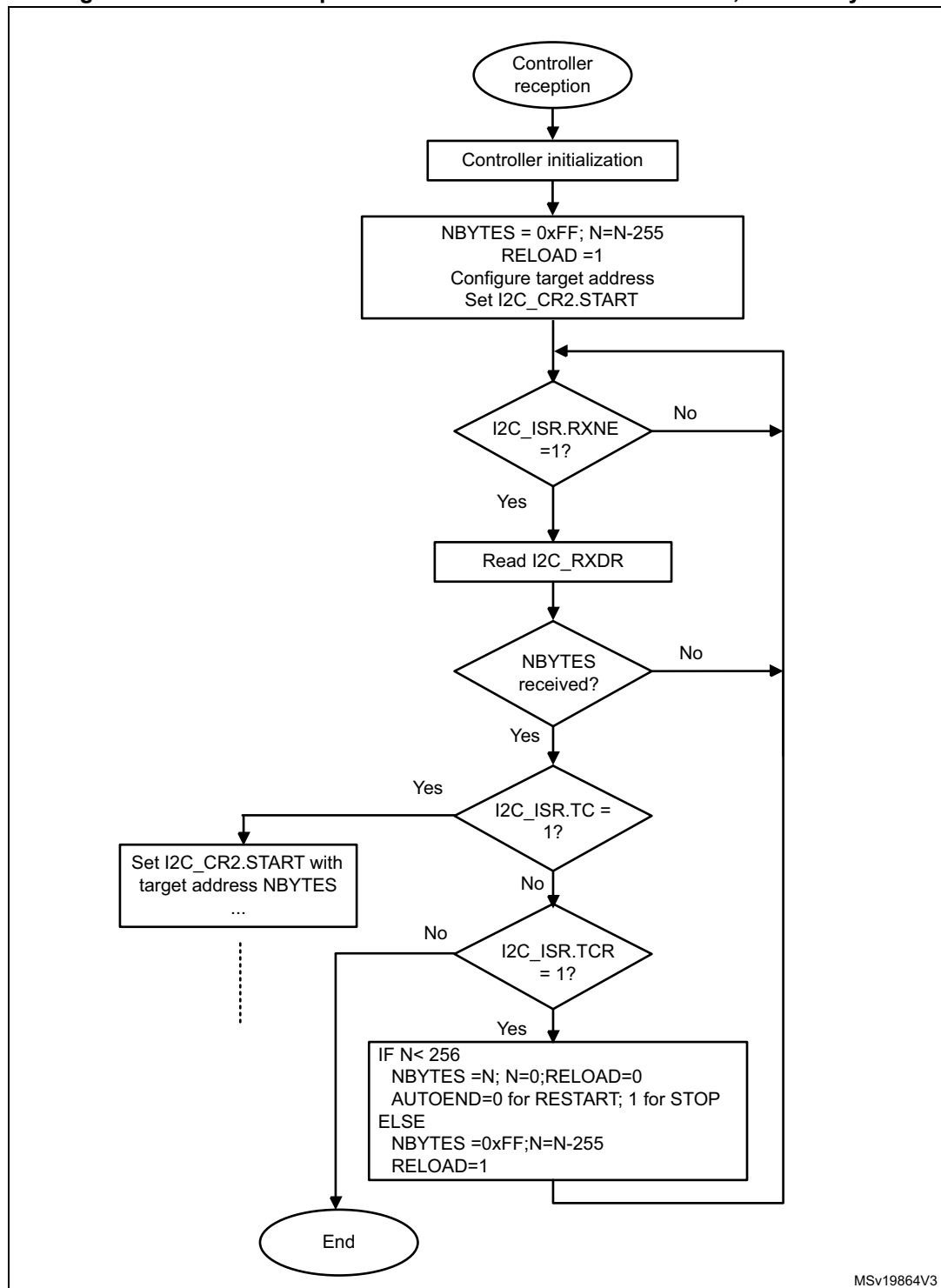
Figure 320. Transfer sequence flow for I2C controller receiver, N &gt; 255 bytes
