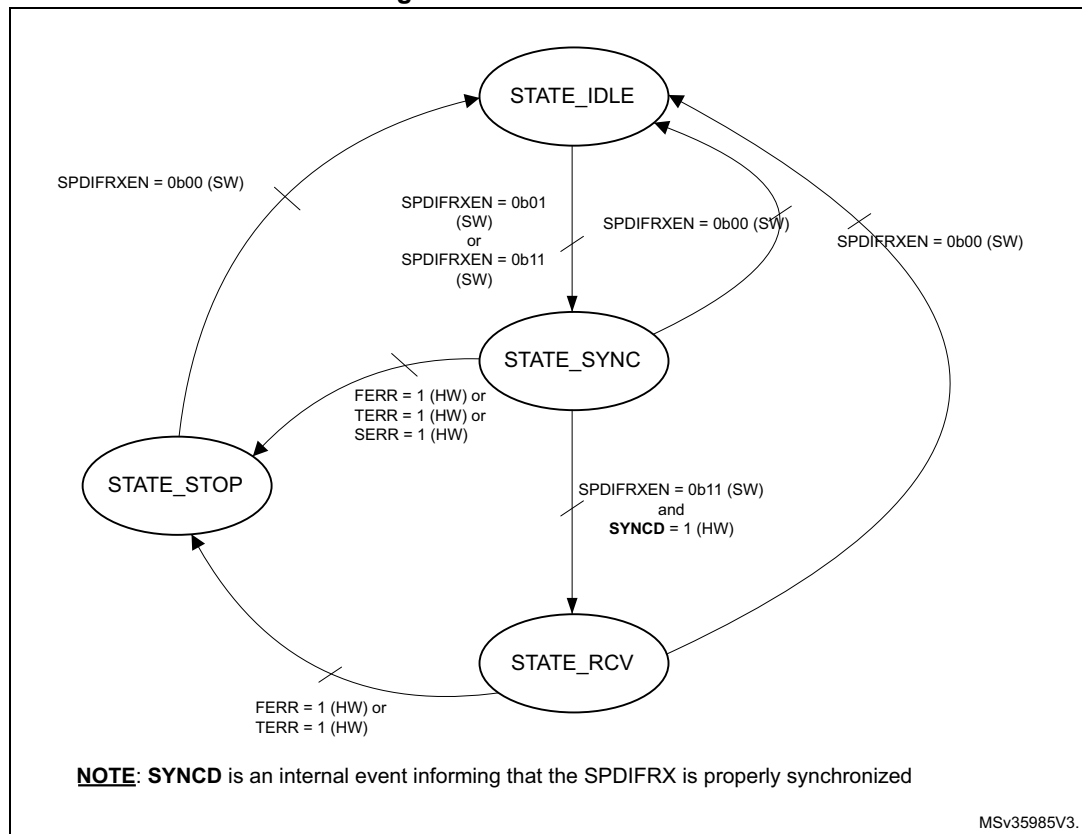
Figure 418. SPDIFRX States
