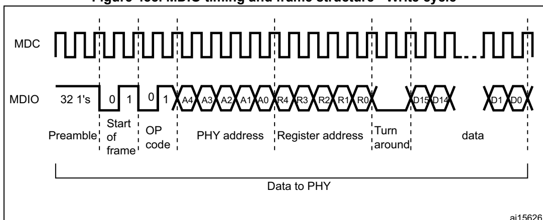
Figure 488. MDIO timing and frame structure - Write cycle
