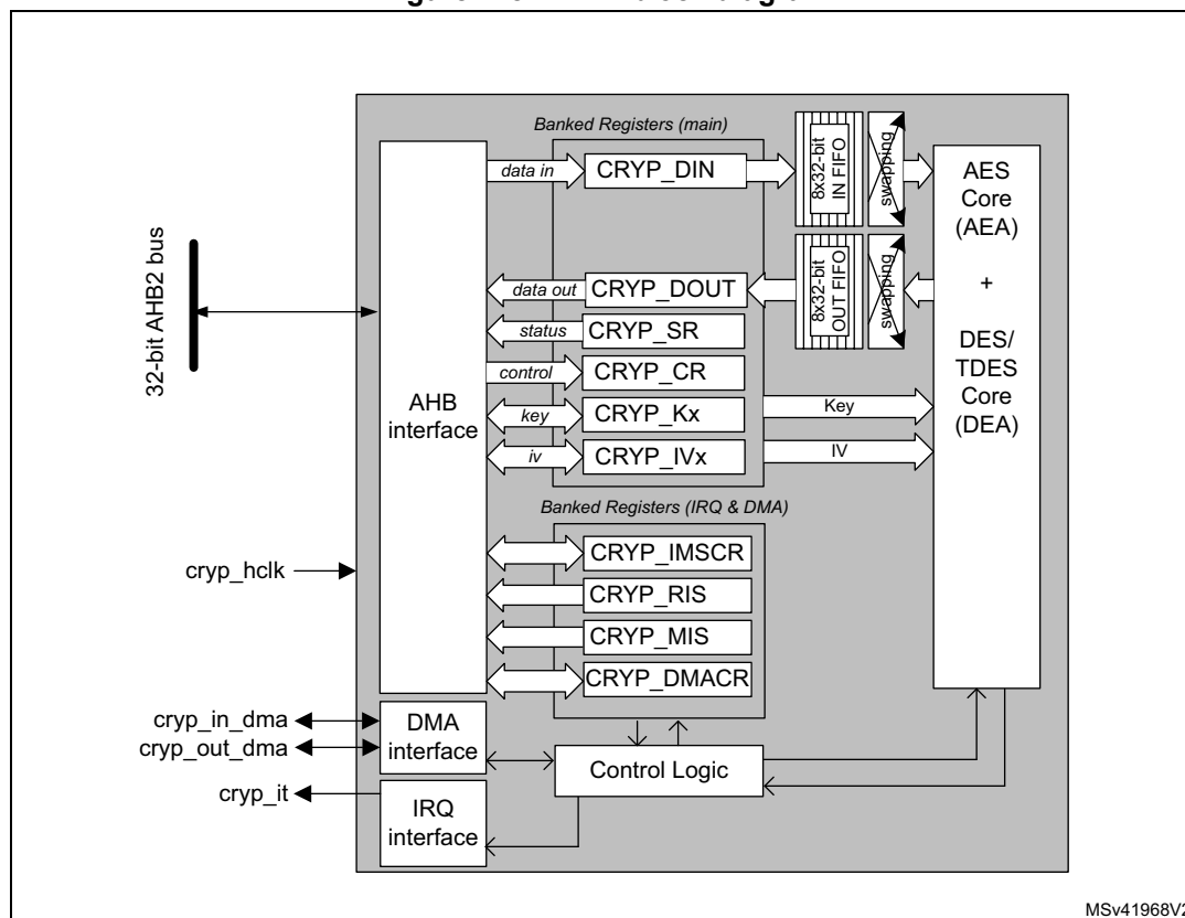
Figure 118. CRYP block diagram
