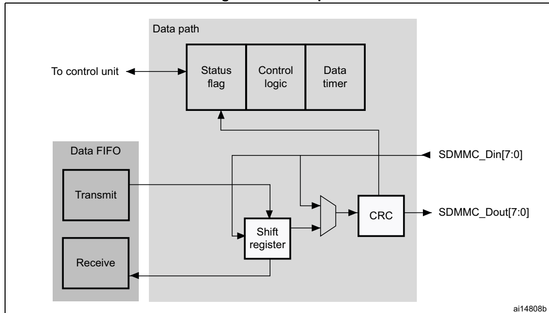
Figure 436. Data path
