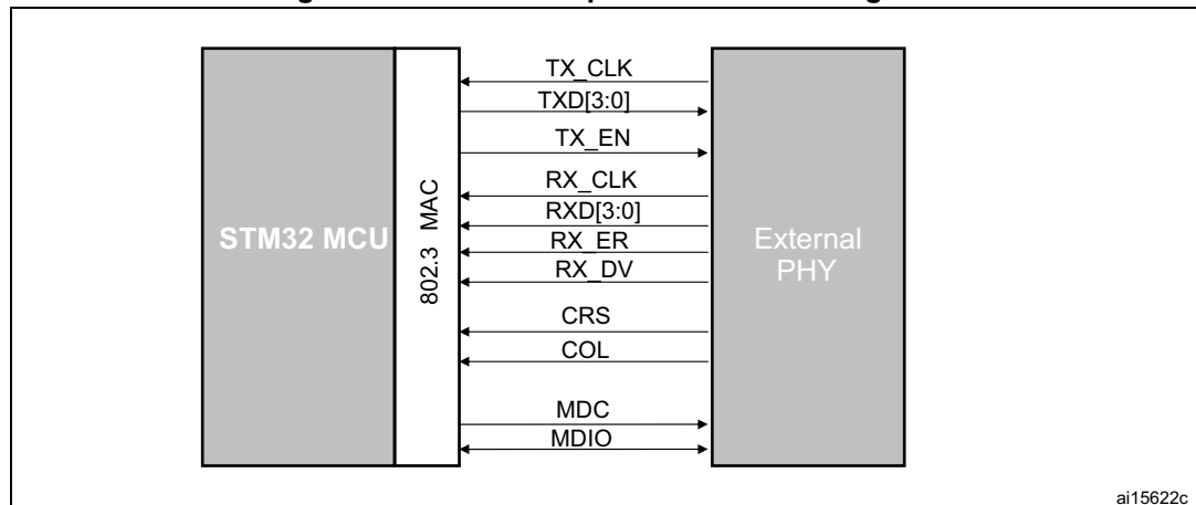
Figure 490. Media independent interface signals
