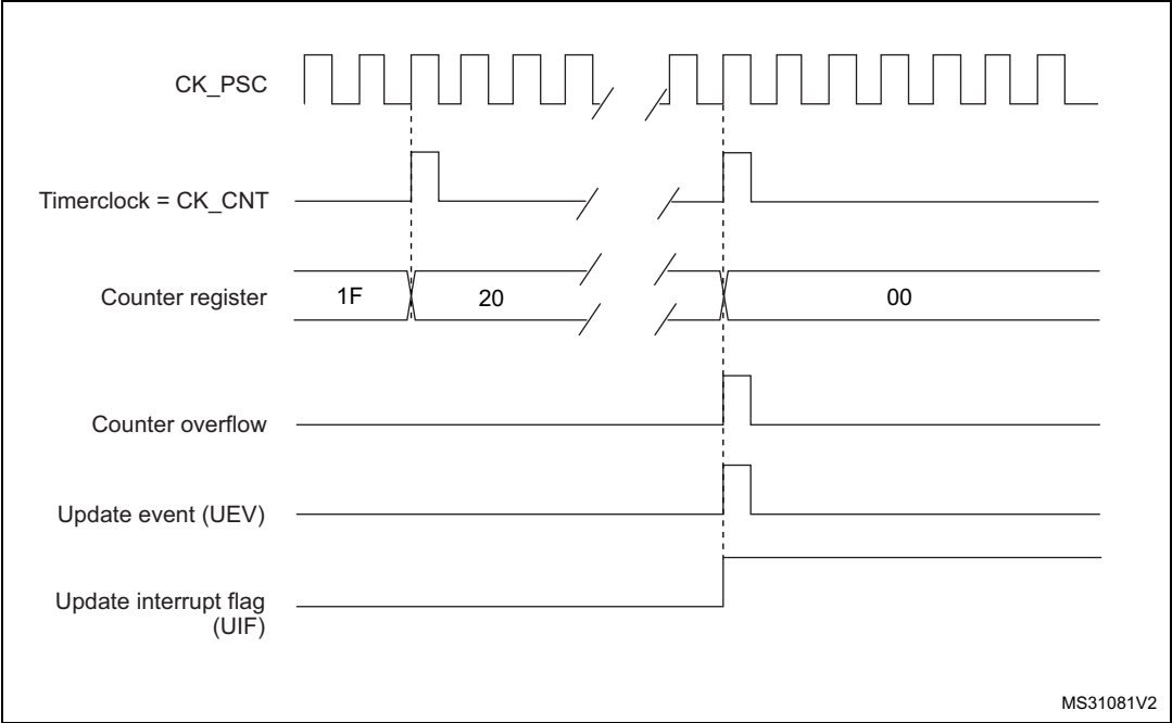
Figure 260. Counter timing diagram, internal clock divided by N
