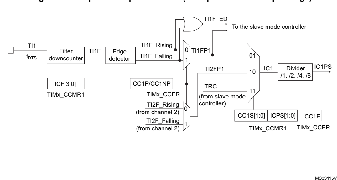
Figure 266. Capture/compare channel (example: channel 1 input stage)
