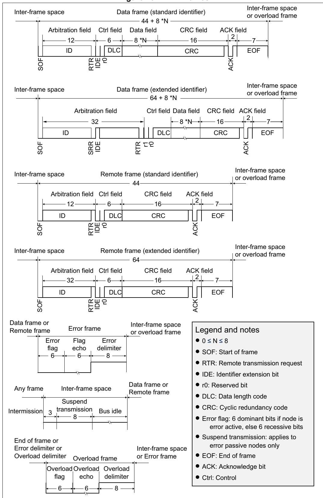
Figure 451. CAN frames
