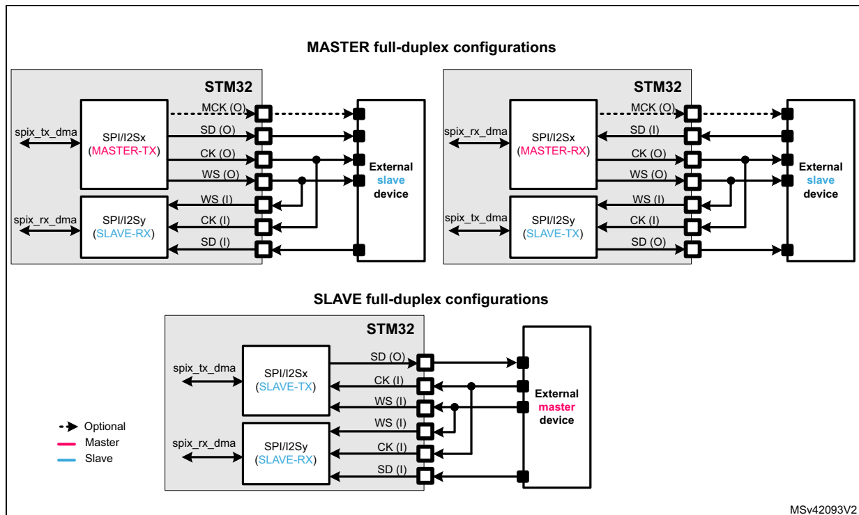
Figure 371. Full-duplex communication
