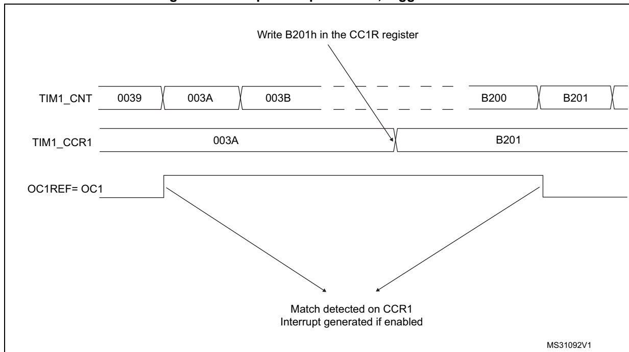
Figure 232. Output compare mode, toggle on OC1
