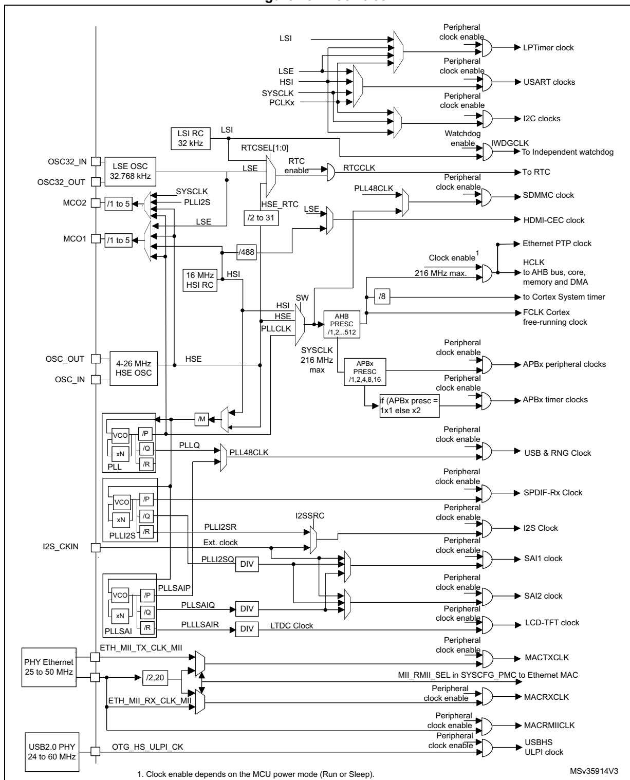
Figure 13. Clock tree
