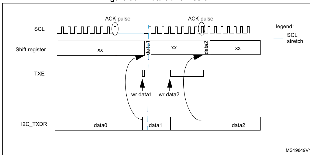
Figure 304. Data transmission
