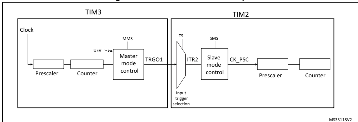
Figure 246. Master/Slave timer example
