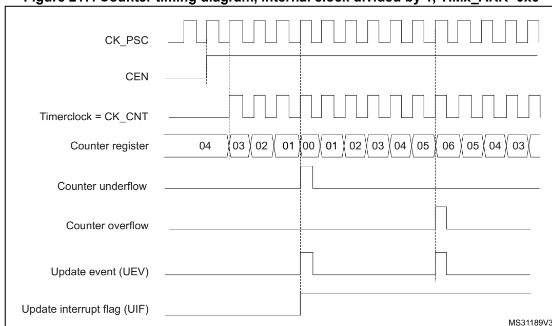
Figure 217. Counter timing diagram, internal clock divided by 1, TIMx_ARR=0x6
