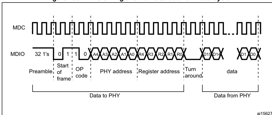
Figure 489. MDIO timing and frame structure - Read cycle
