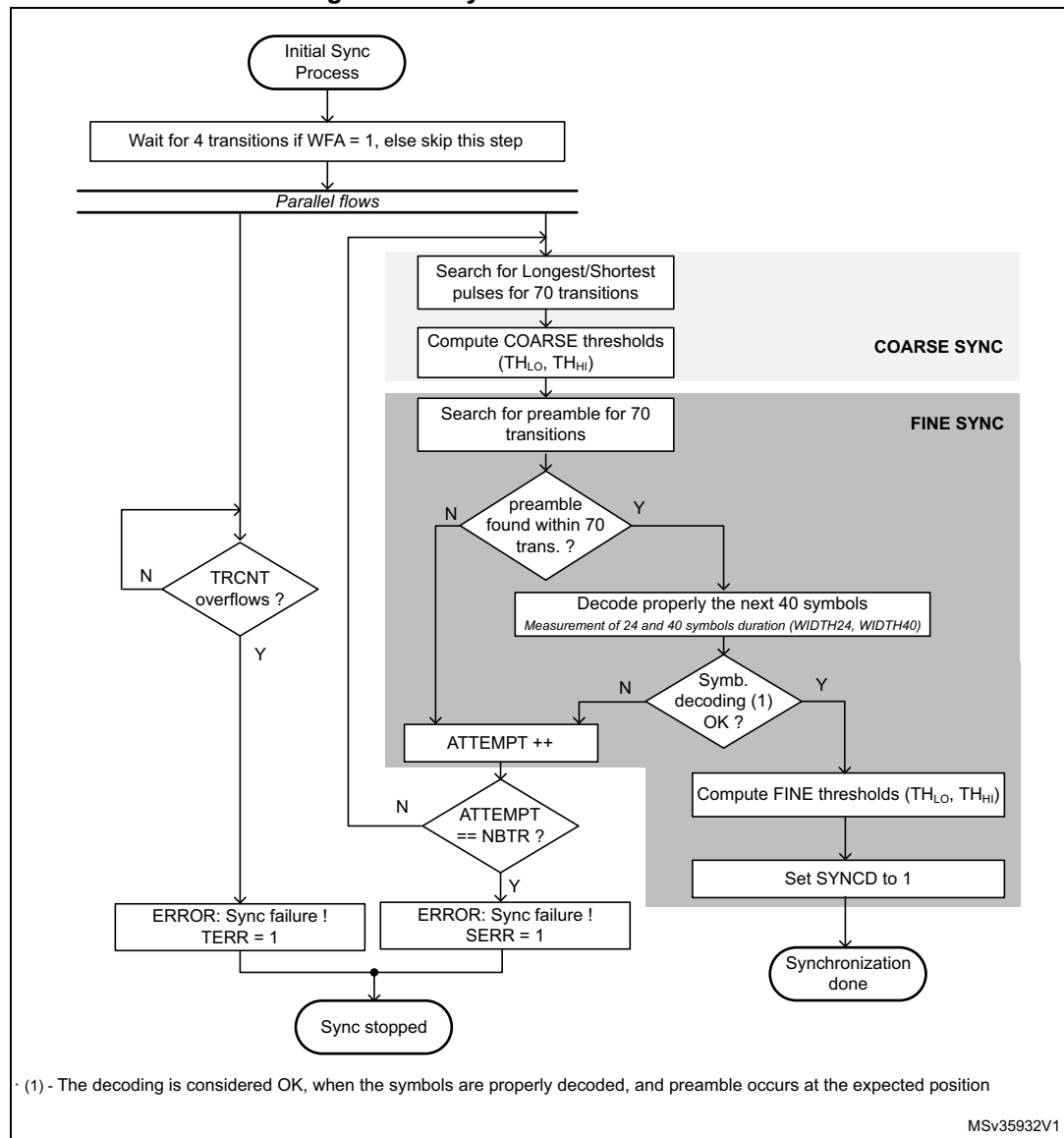
Figure 416. Synchronization flowchart
