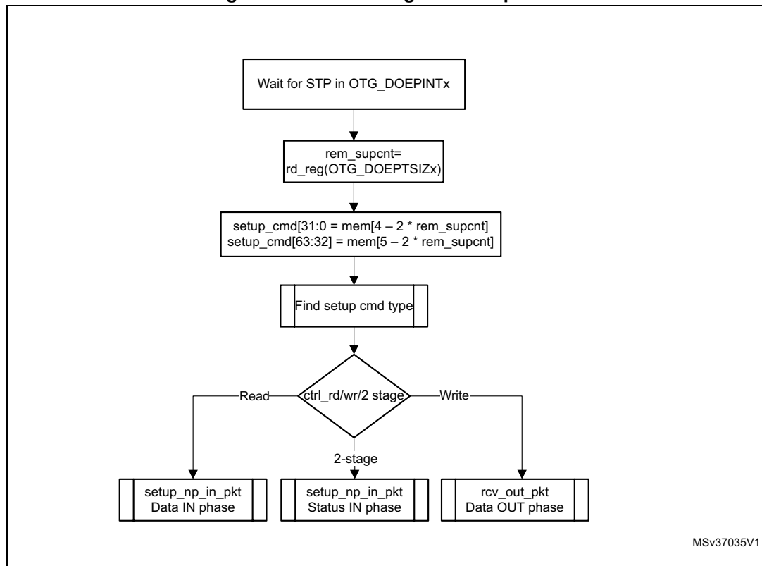
Figure 479. Processing a SETUP packet
