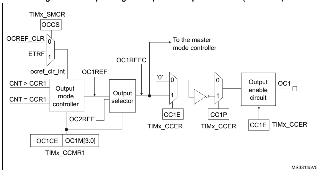
Figure 230. Output stage of Capture/Compare channel (channel 1)
