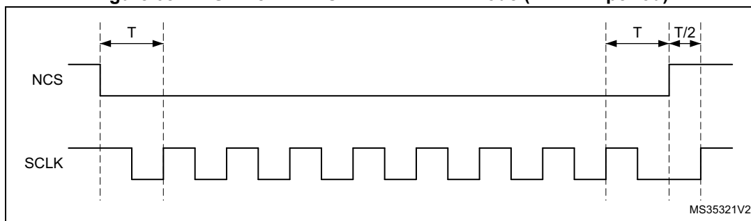
Figure 68. NCS when CKMODE = 1 in DDR mode ( T = \text{CLK period} )
