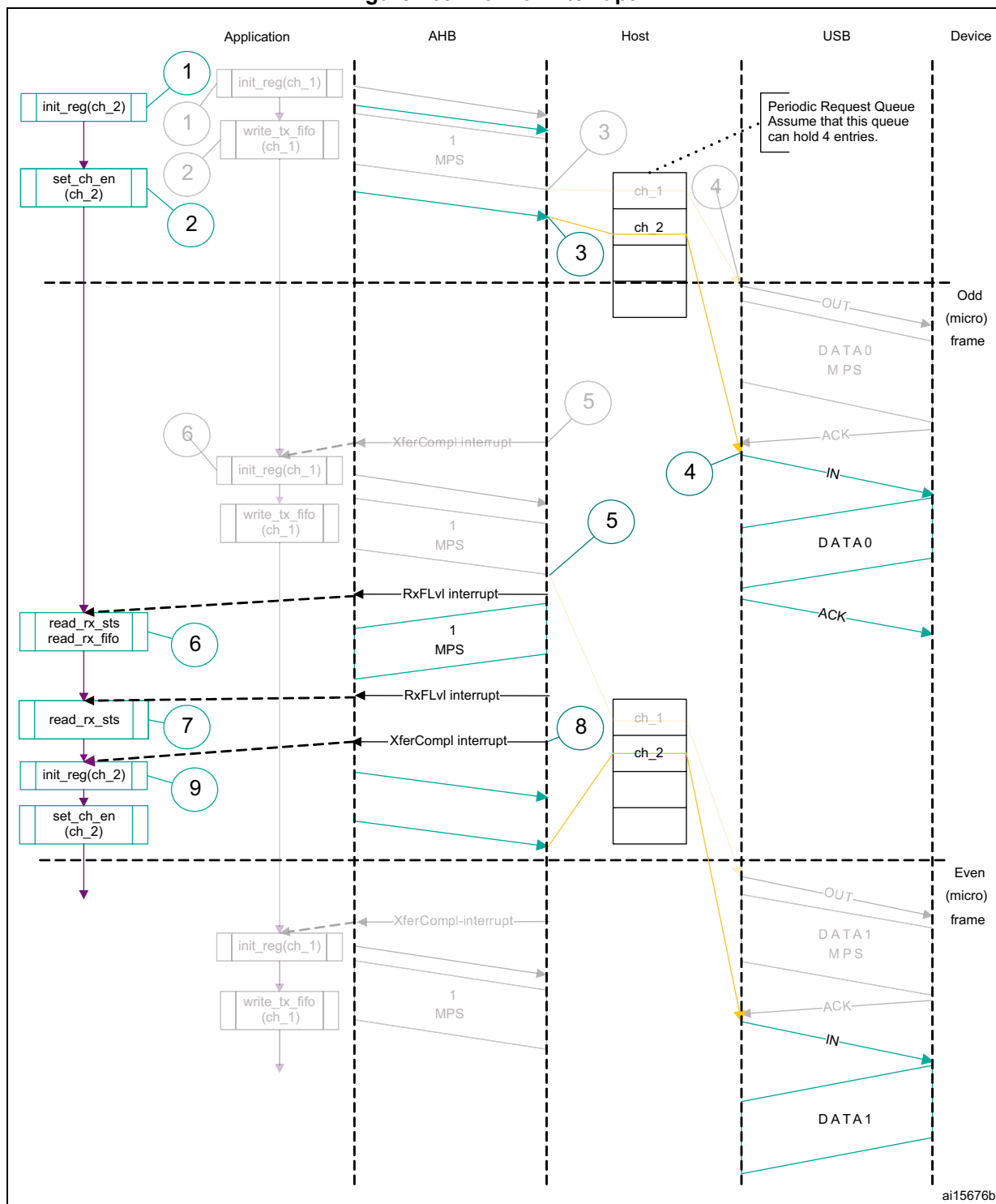
Figure 469. Normal interrupt IN
