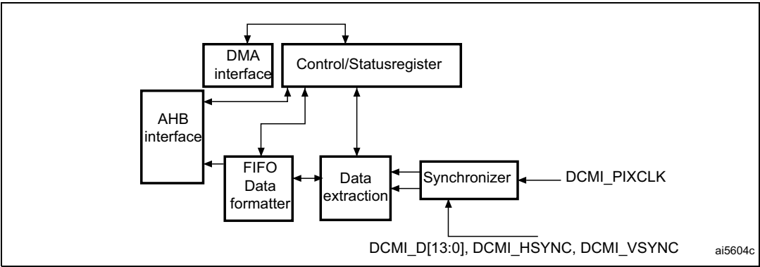
Figure 103. Top-level block diagram
