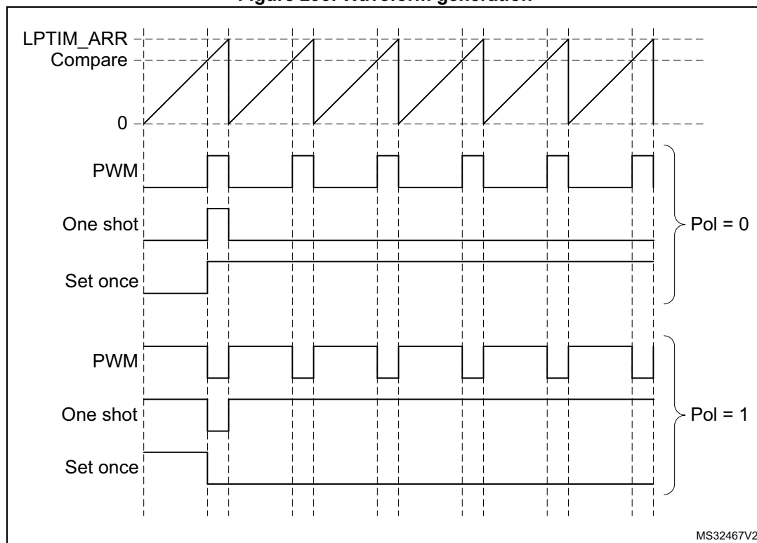
Figure 293. Waveform generation
