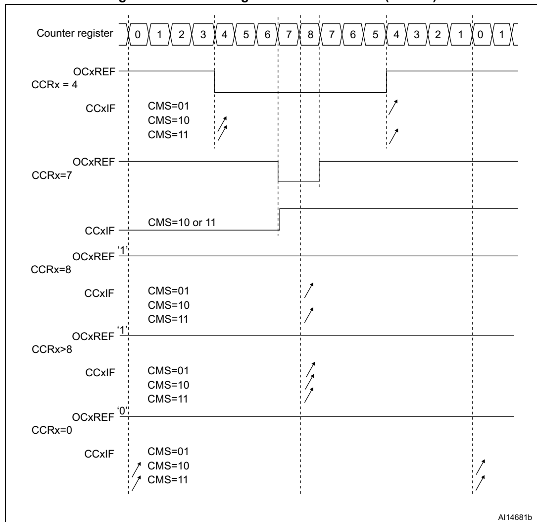
Figure 234. Center-aligned PWM waveforms (ARR=8)
