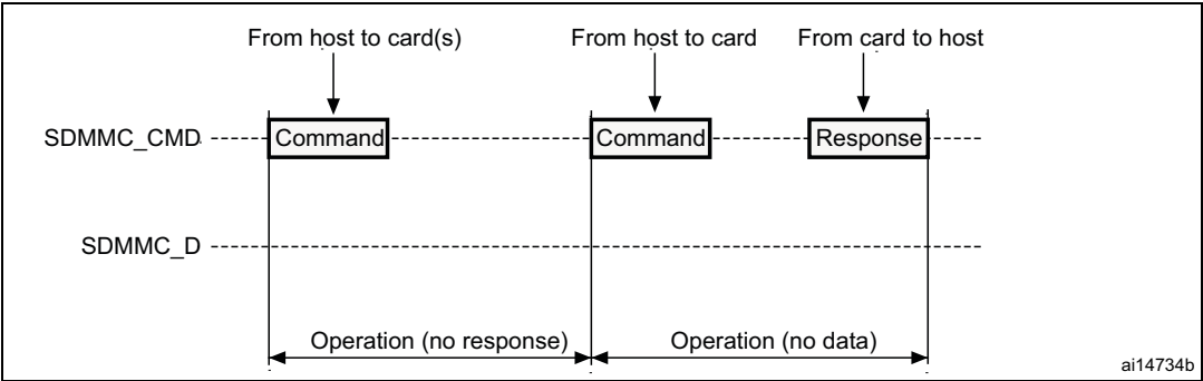
Figure 424. “No response” and “no data” operations
