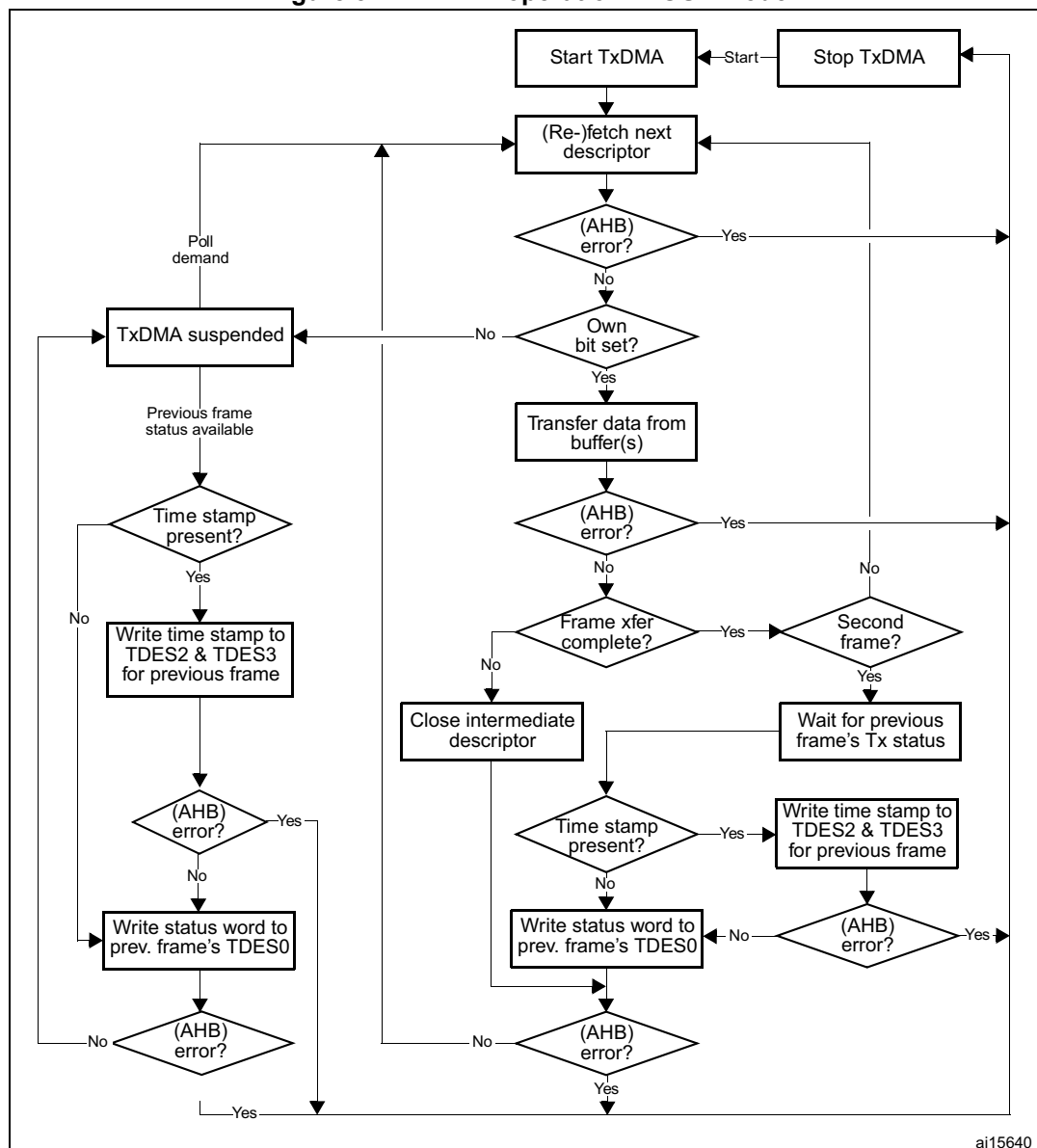
Figure 514. TxDMA operation in OSF mode
