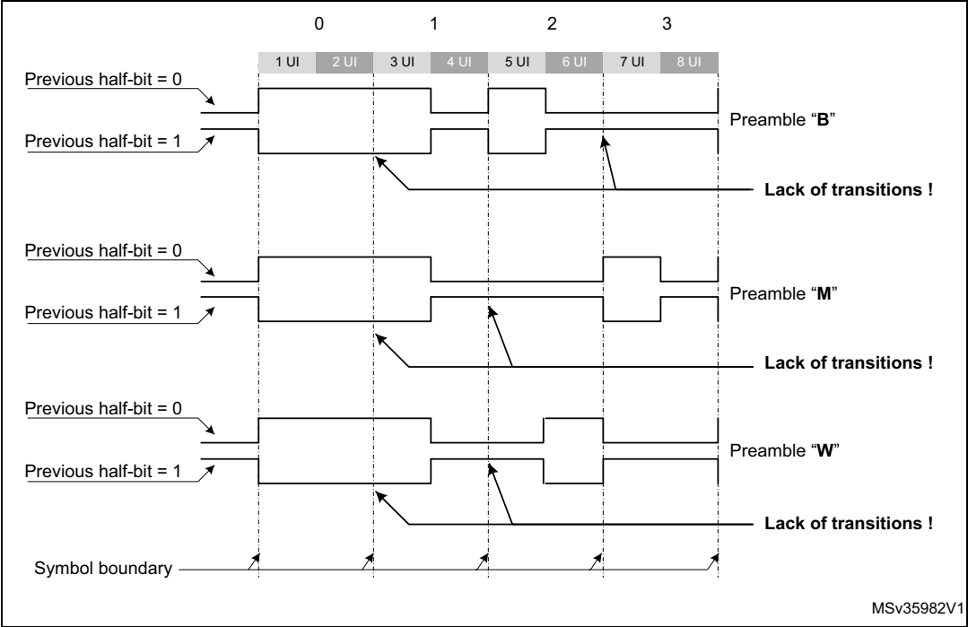
Figure 411. S/PDIF Preambles
