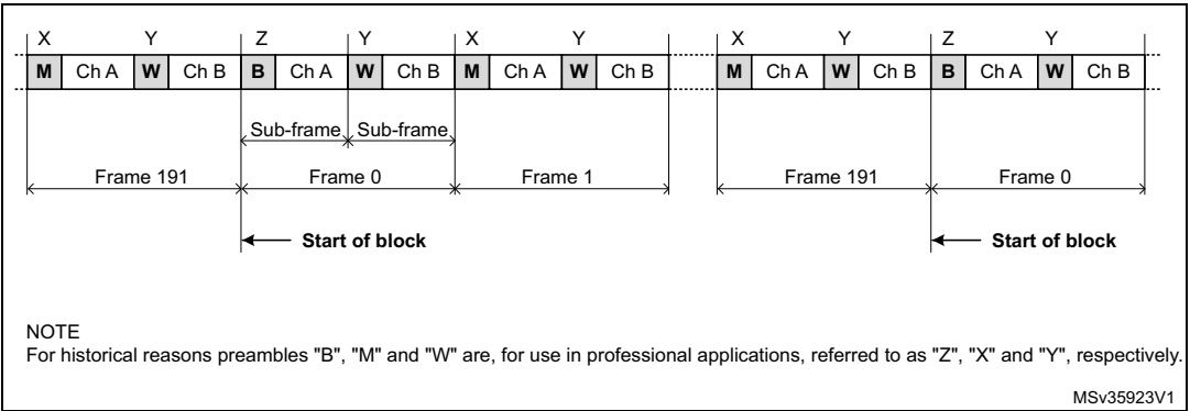
Figure 410. S/PDIF block format
