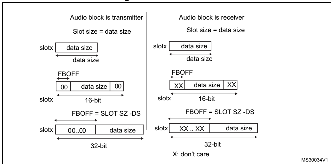
Figure 397. First bit offset
