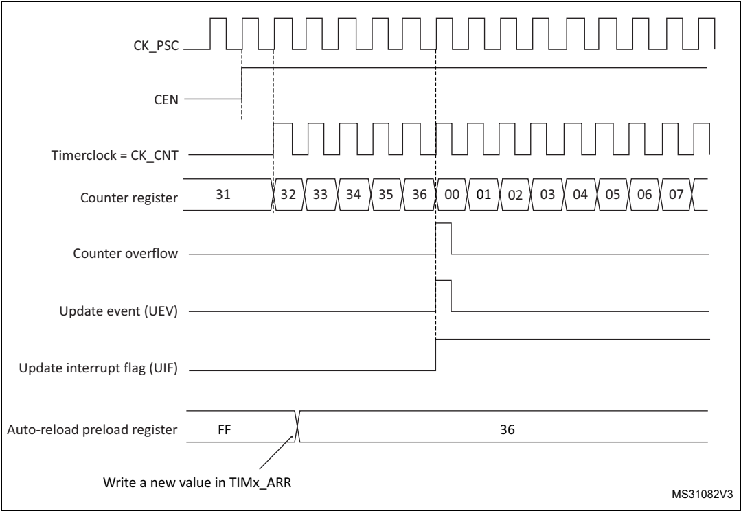
Figure 152. Counter timing diagram, update event when ARPE=0 (TIMx_ARR not preloaded)
