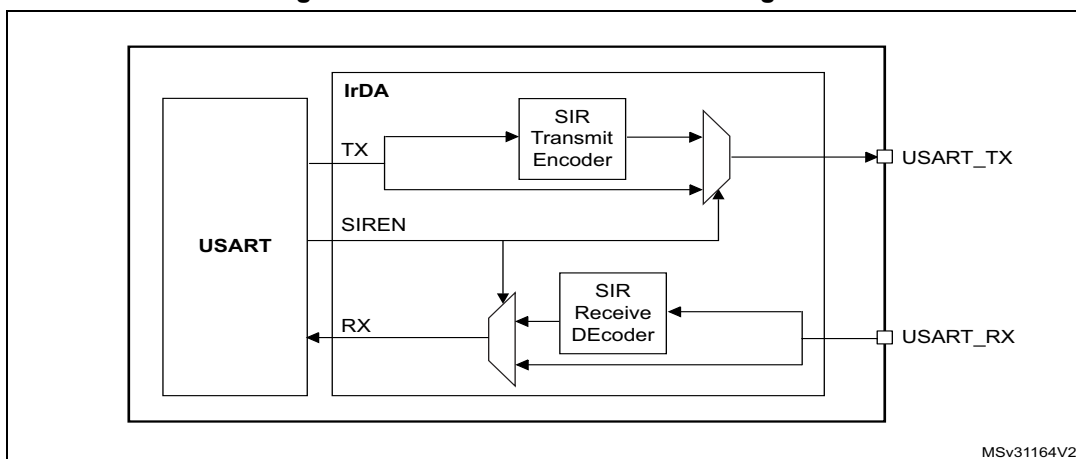
Figure 346. IrDA SIR ENDEC- block diagram
