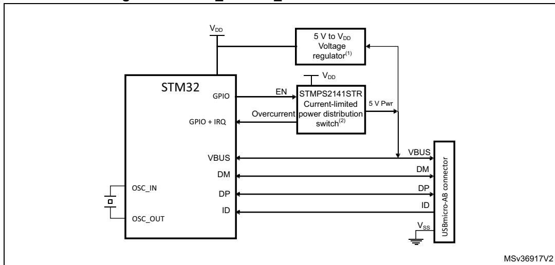
Figure 456. OTG_FS/OTG_HS A-B device connection
