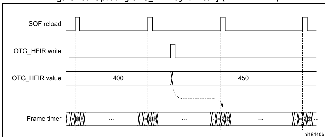
Figure 460. Updating OTG_HFIR dynamically (RLDCTRL = 1)
