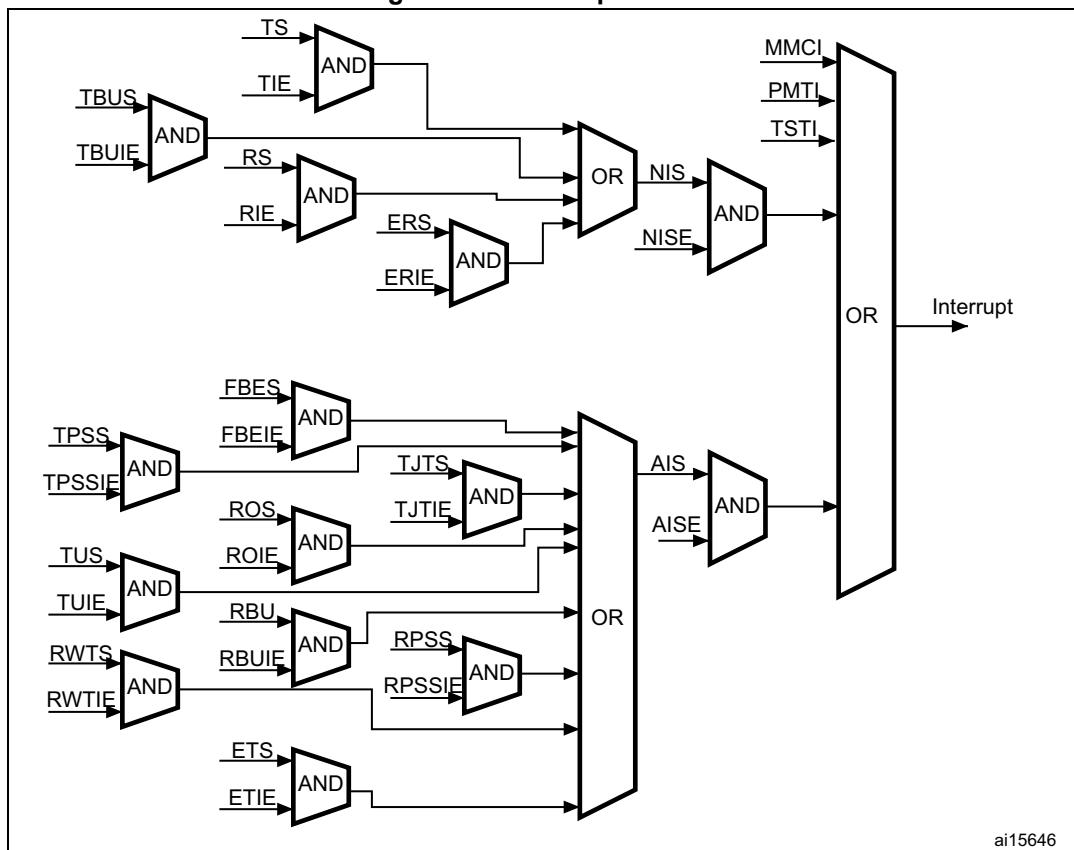
Figure 520. Interrupt scheme
