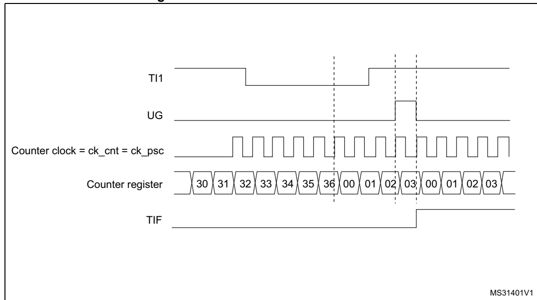
Figure 199. Control circuit in reset mode
