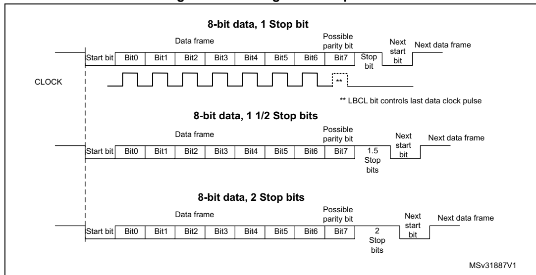
Figure 331. Configurable stop bits
