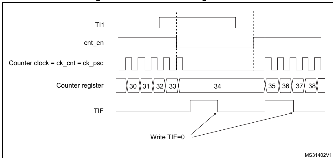
Figure 276. Control circuit in gated mode
