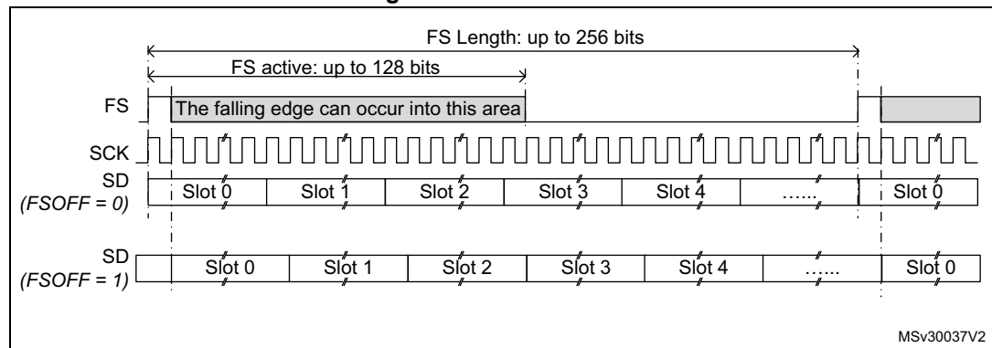
Figure 393. Audio frame
