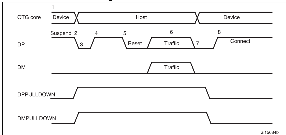
Figure 485. B-device HNP
