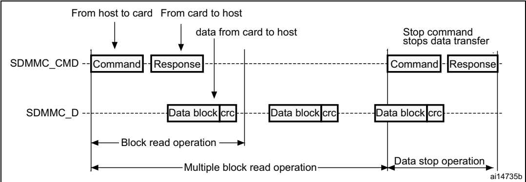
Figure 425. (Multiple) block read operation
