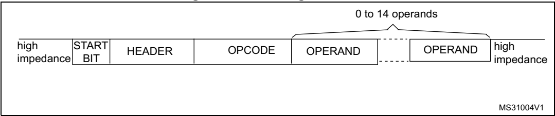
Figure 523. Message structure
