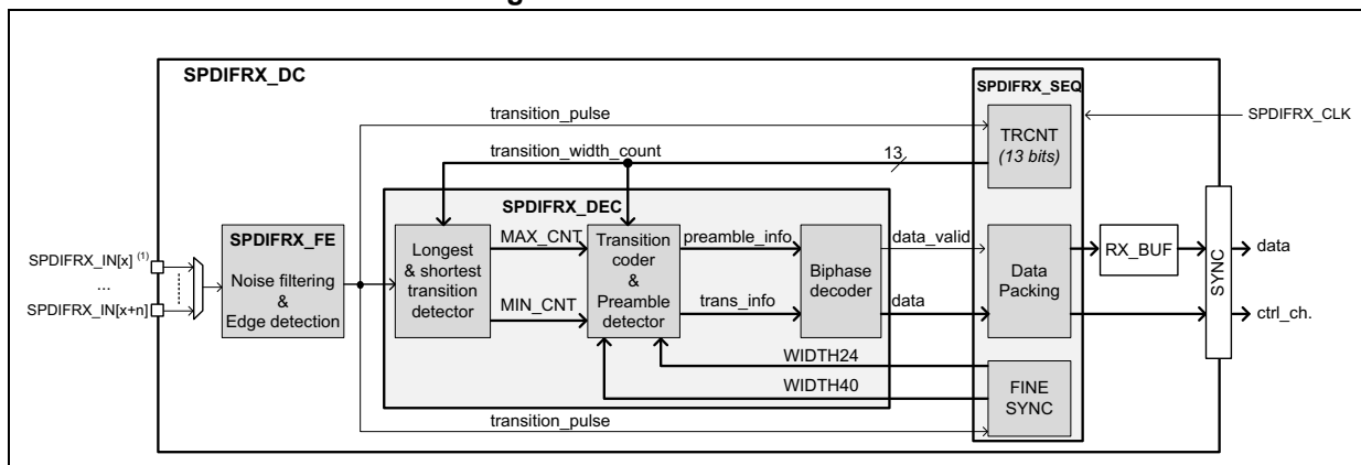
Figure 413. SPDIFRX decoder
