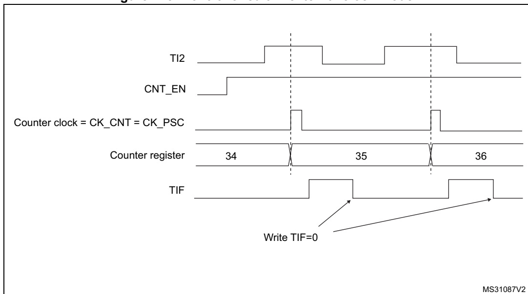
Figure 225. Control circuit in external clock mode 1
