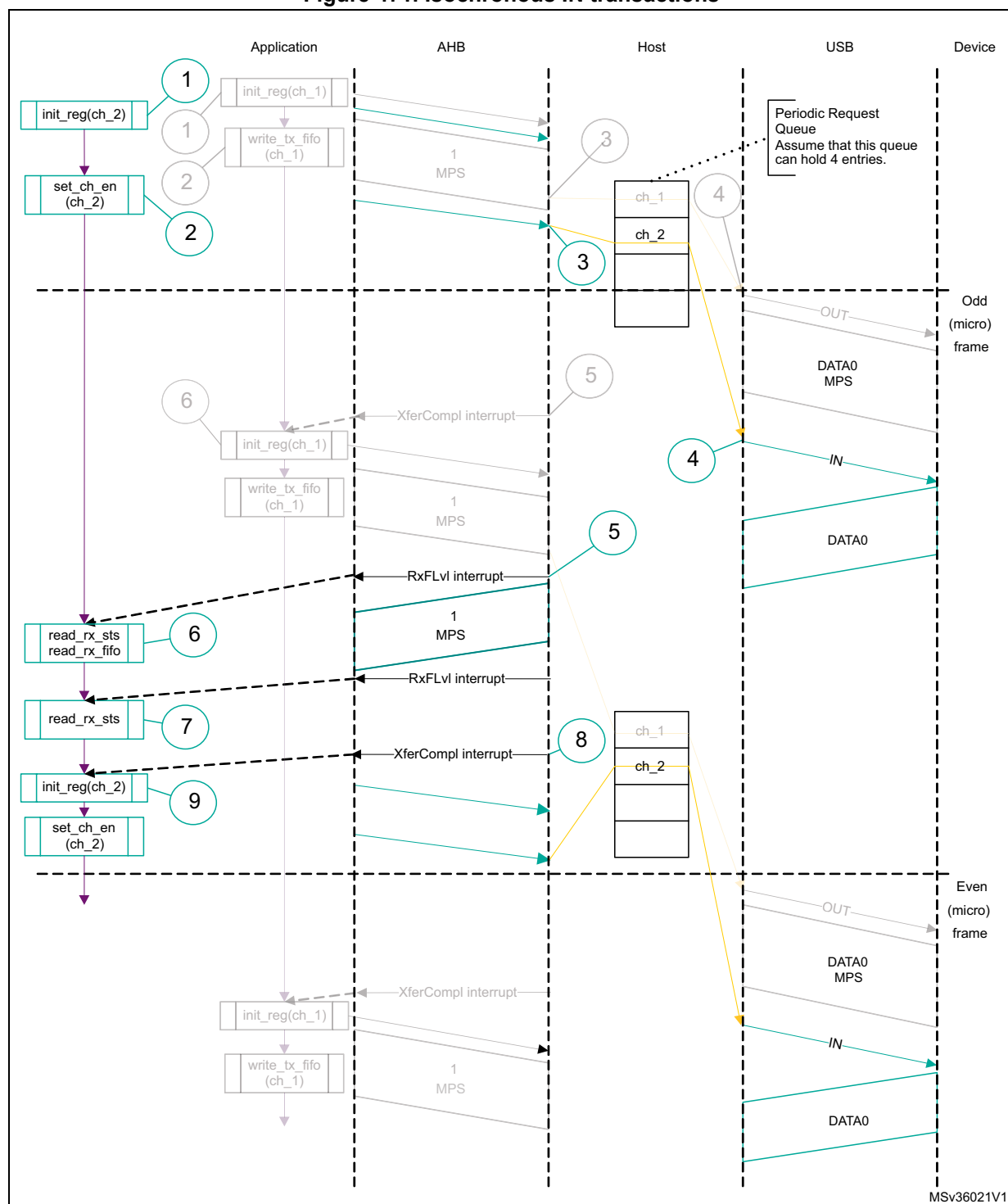
Figure 471. Isochronous IN transactions
