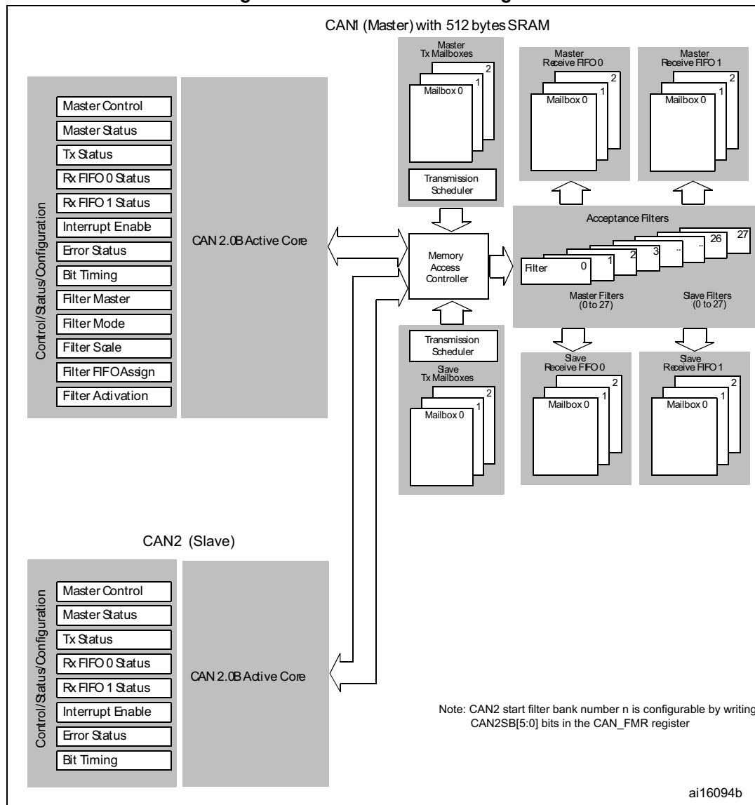
Figure 439. Dual-CAN block diagram
