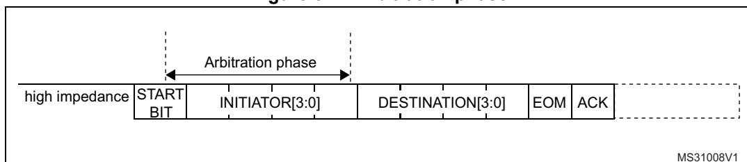
Figure 527. Arbitration phase
