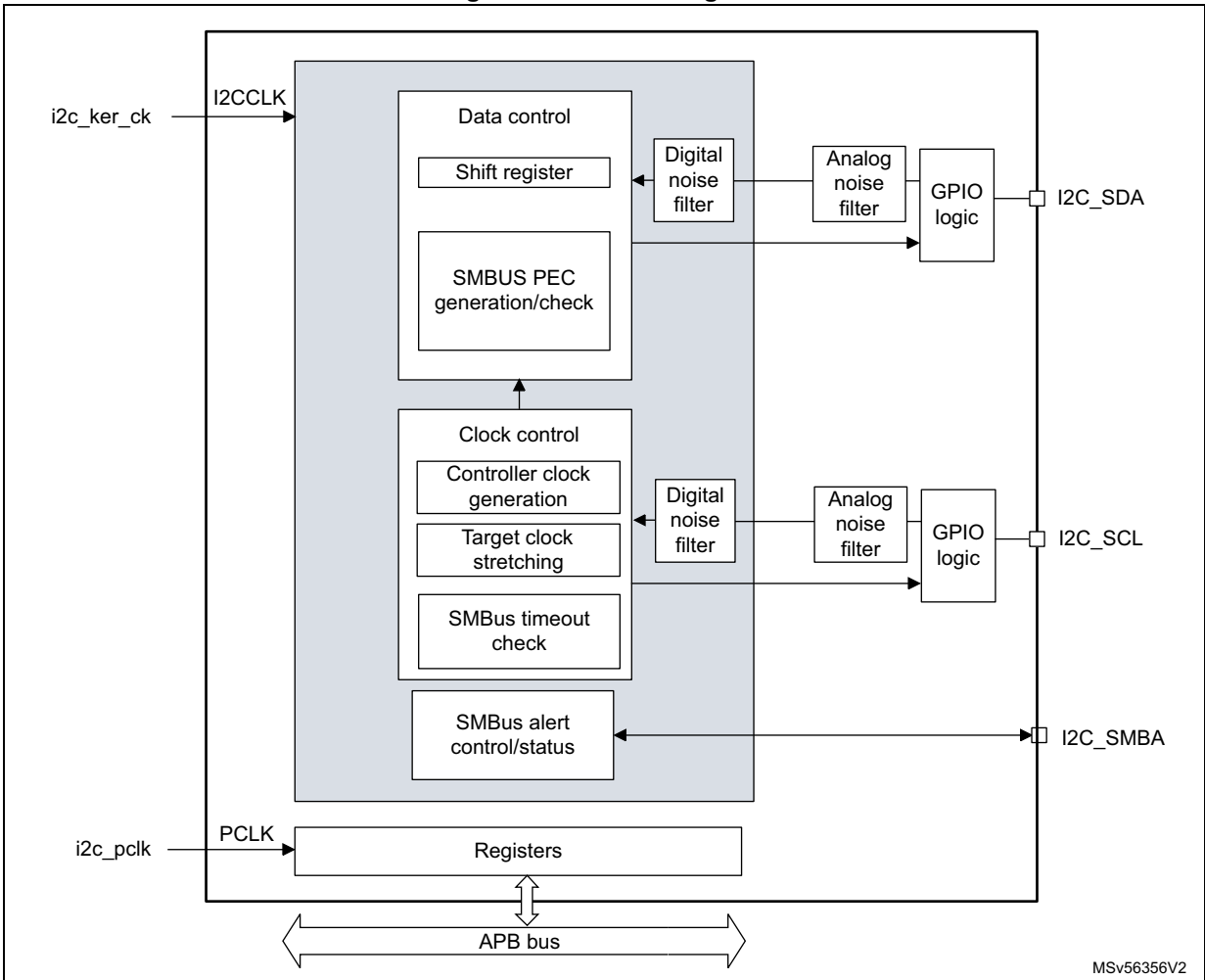
Figure 299. Block diagram
