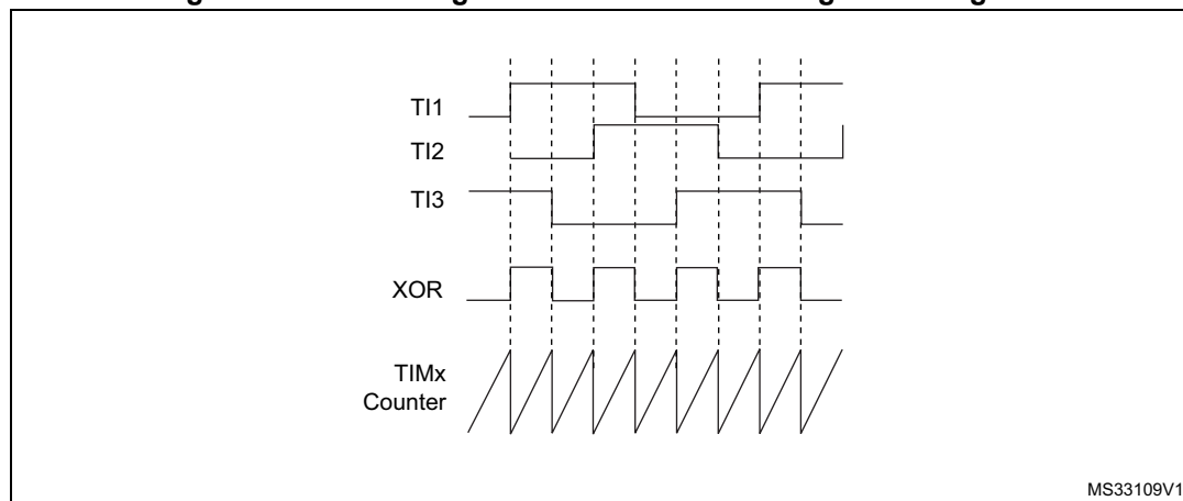
Figure 197. Measuring time interval between edges on 3 signals
