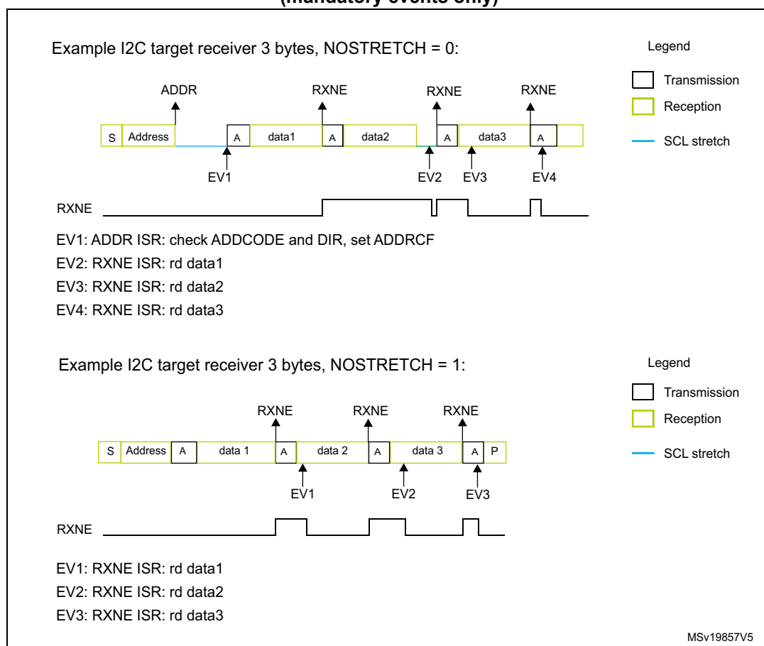
Figure 311. Transfer bus diagrams for I2C target receiver (mandatory events only)
