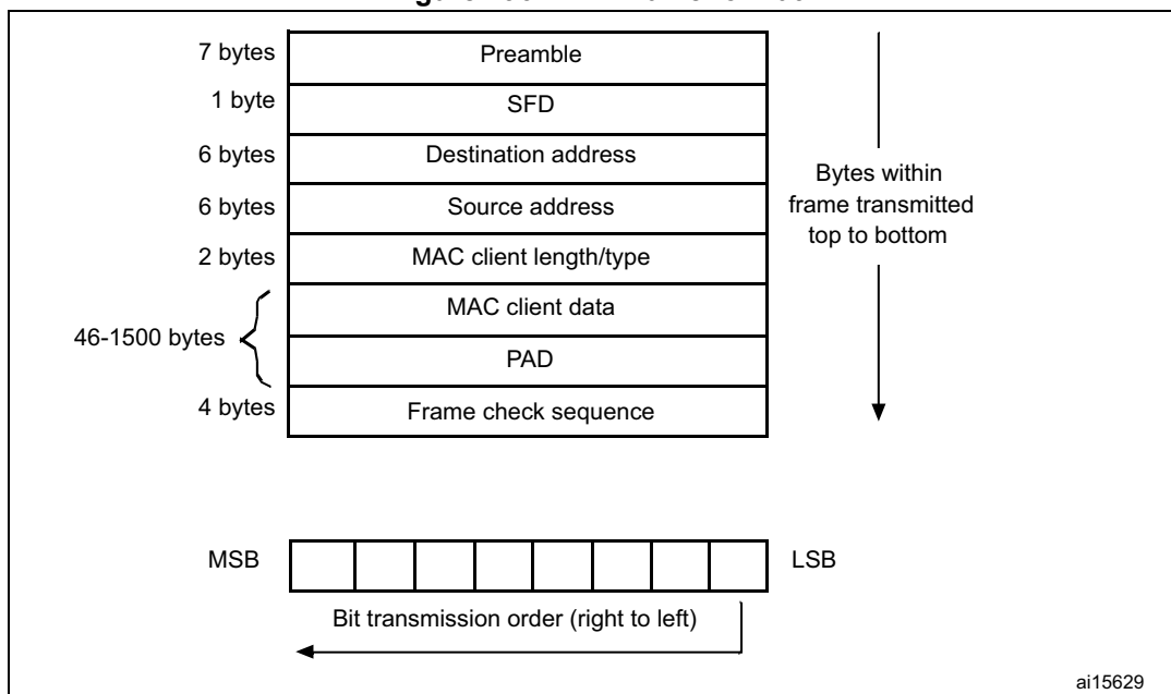
Figure 496. MAC frame format
