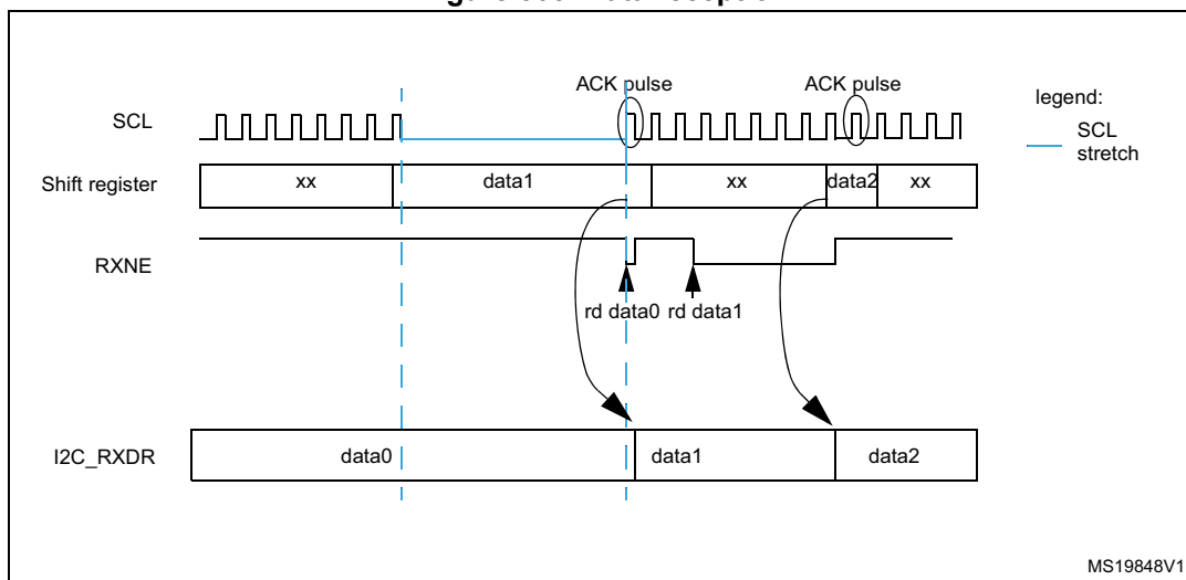
Figure 303. Data reception
