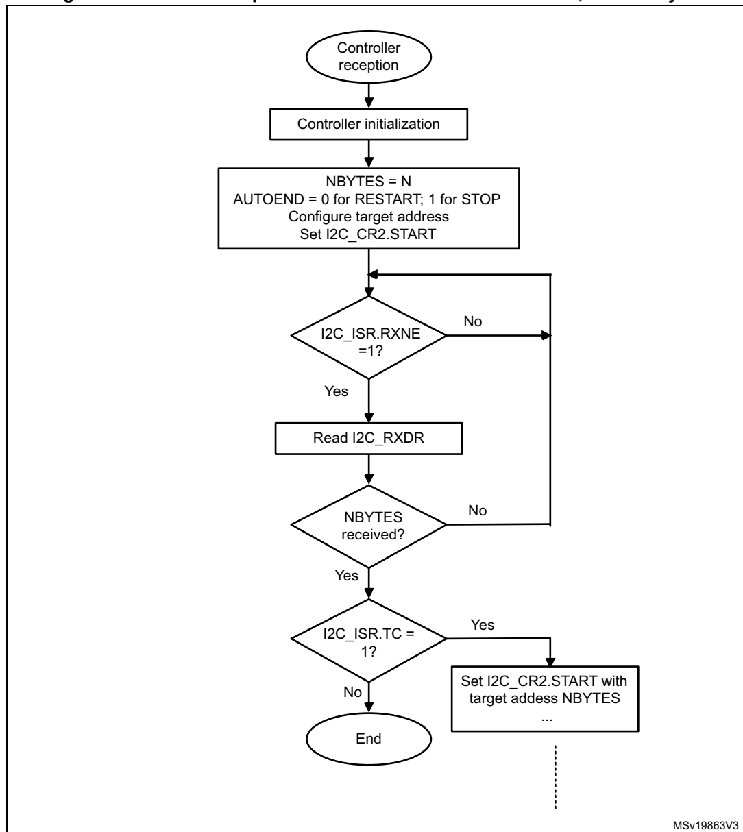
Figure 319. Transfer sequence flow for I2C controller receiver, N \leq 255 bytes
